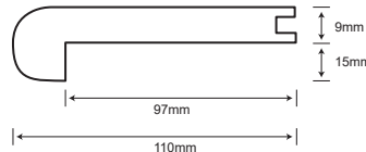
FLUSH STAIR NOSE
